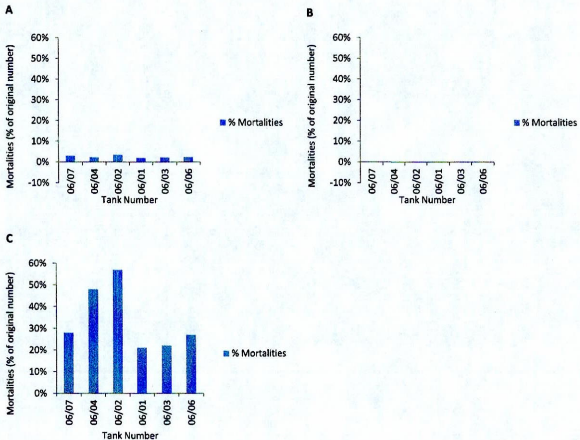
Figure A2. Shellfish mortalities (percentage) during the experimental work. A: mussels; B: Pacific oysters; C: cockles. Tank numbers and corresponding target water concentration (cfu E. coli /100ml) 06/07 = 1; 06/04 = 3.3; 06/02 = 10; 06/01 = 33; 06/03 = 100; 06/06 = 300.
